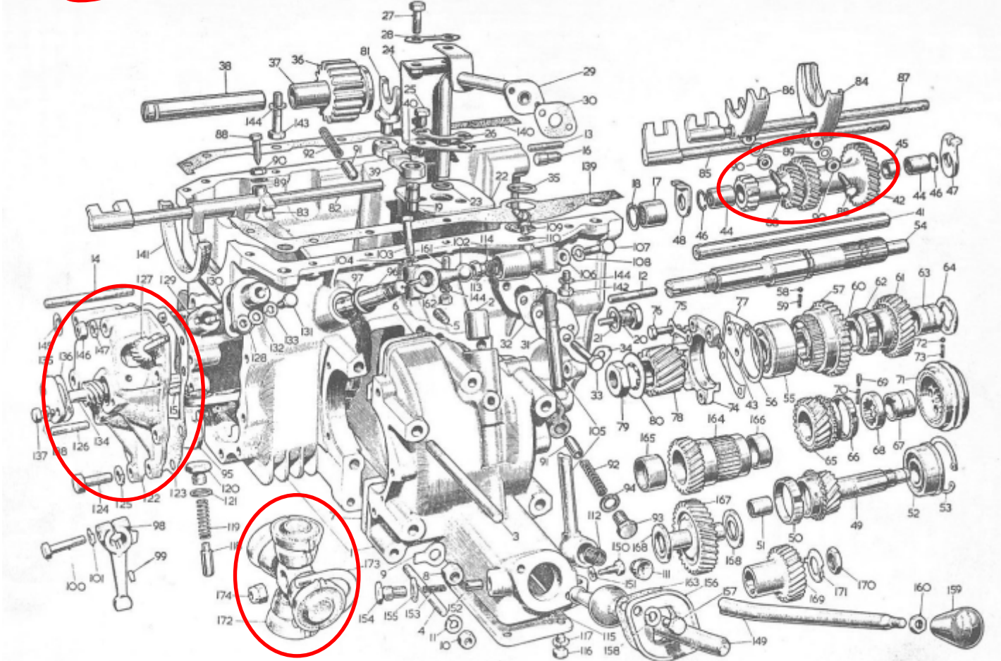
FIG 6-4 Component parts of the transmission
